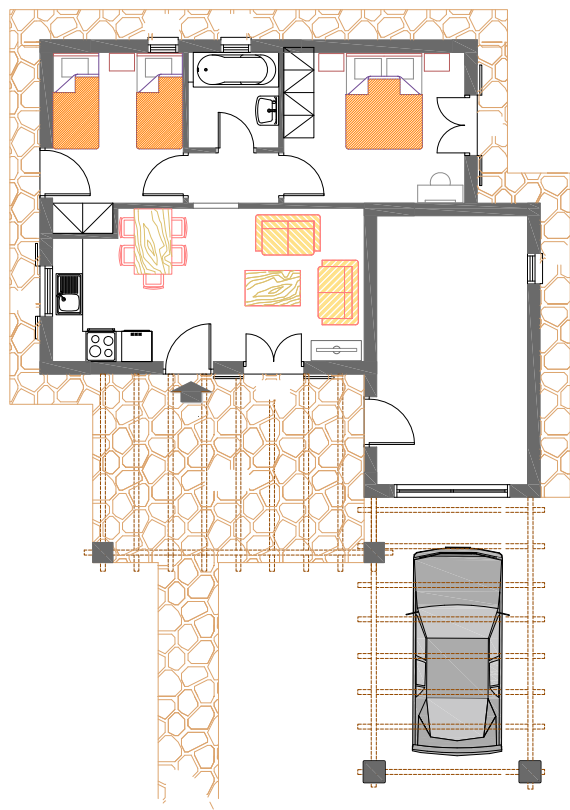
FLOOR PLAN
